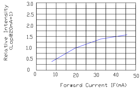
Relative Luminous intensity vs Forward current
