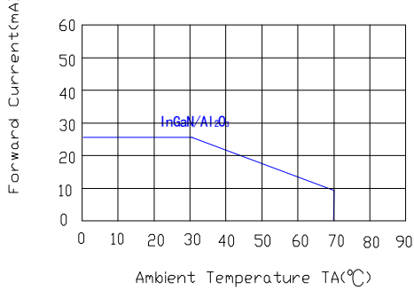
Forward Current Denating Curve
