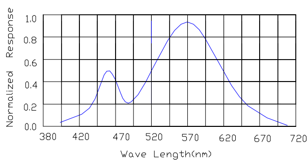
Spectral Reduance
