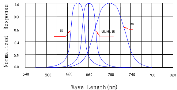
Spectral Reduance
