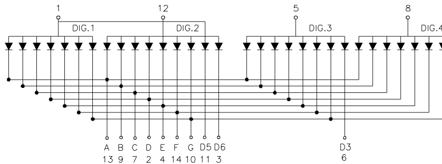
Common Anode
