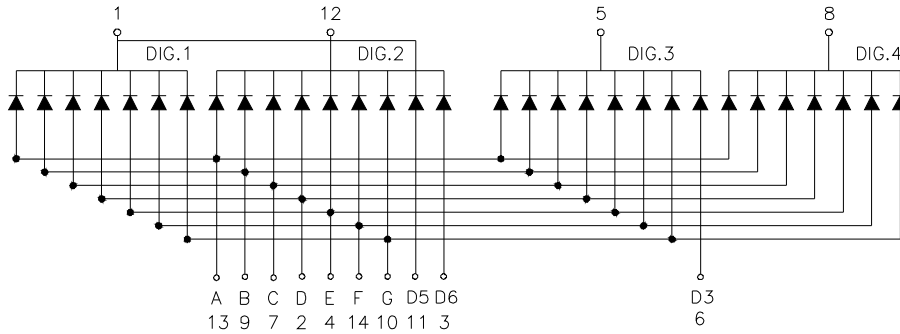
Common Cathode
