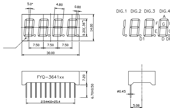
FYQ-3641 Series
